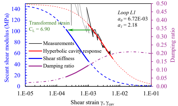
Figure 10. Interpretation of loop L1 (dense sands).
